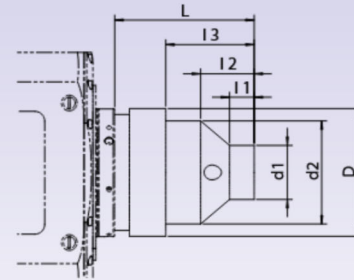
Mounting chuck, automatic Type B axfix
