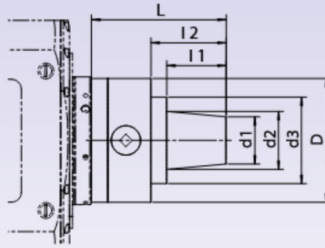
Mounting chuck, manual
